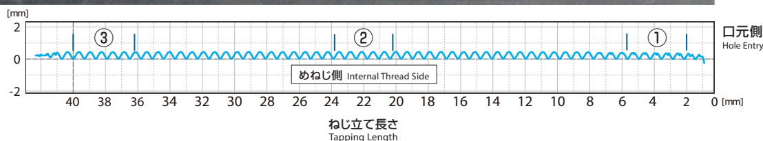
ねじ部拡大 Close-up of Thread Section
